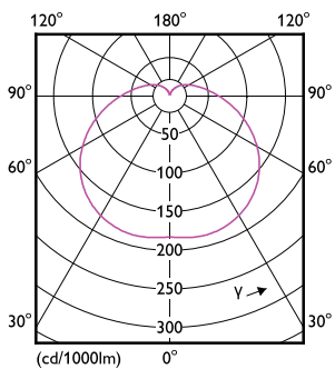
LEDForce HB 55W Tshape E27
